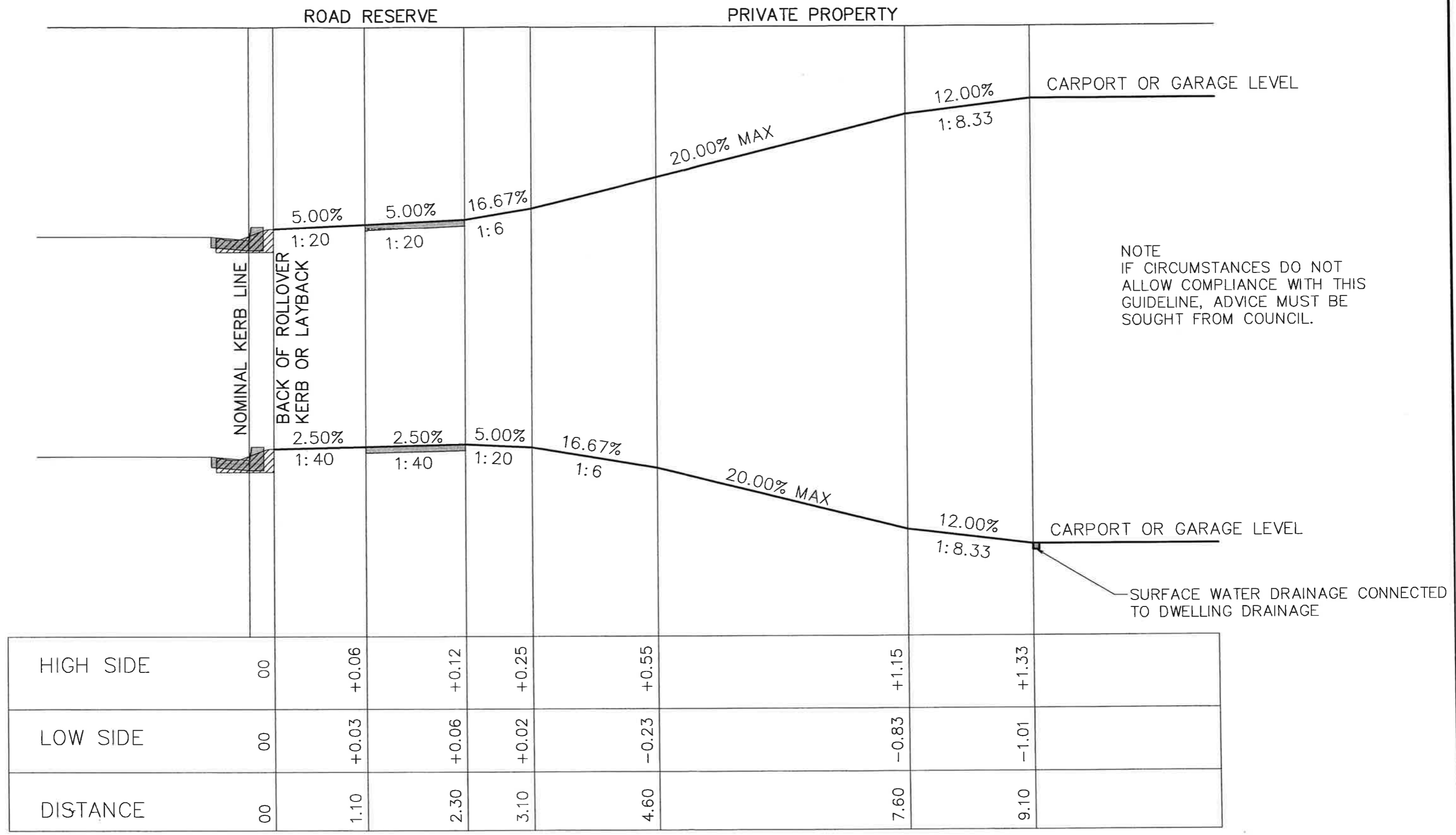
GUIDELINE FOR HIGH & LOW DRIVEWAY PROFILE 1:50
